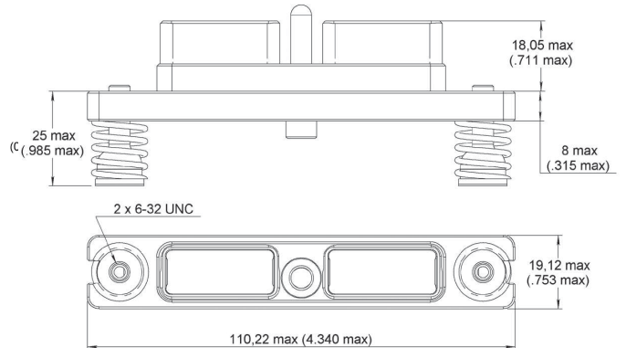
Rear Mount
