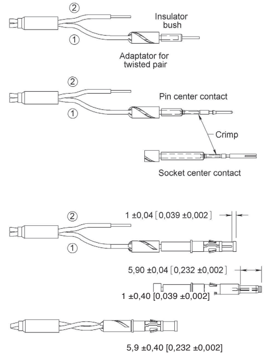
PIN CONTACT
