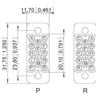
14 CONTACTS
