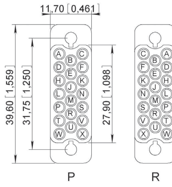
20 CONTACTS
